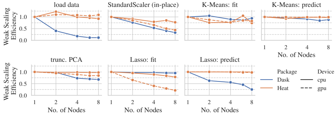
Figure 4: Weak scaling efficiency of typical ML operations in Heat (CPU and GPU) and Dask (CPU). The (dashed) lines show the geometric mean of the observed values. (Higher values are better.)
