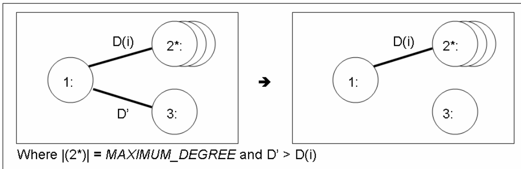
Figure 6: Too many communication partners: the most remote one is abandoned. Classical graph transformation systems, without counting features, cannot process such kind of rules.
