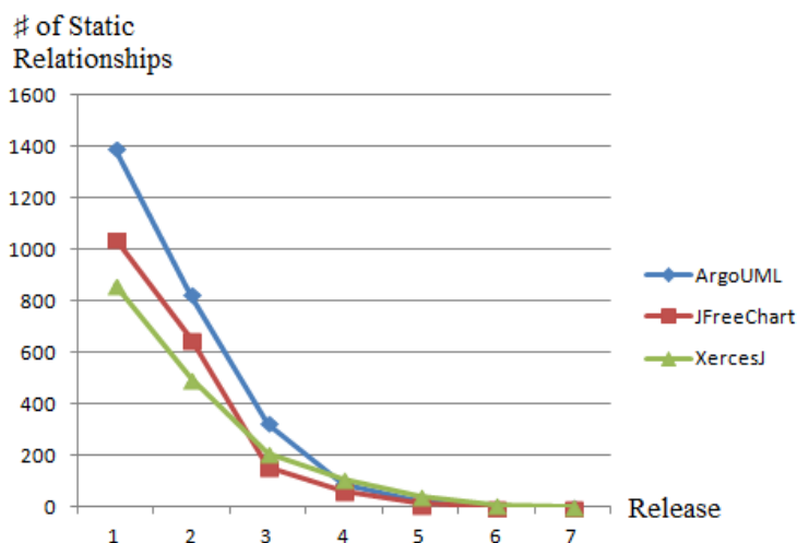
Figure 2: The persistence of static relationships detected in the first software version between anti-patterns and designs patterns.
