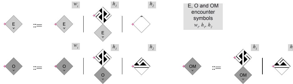
Figure 8: Transducer rules to grow a design vertically
