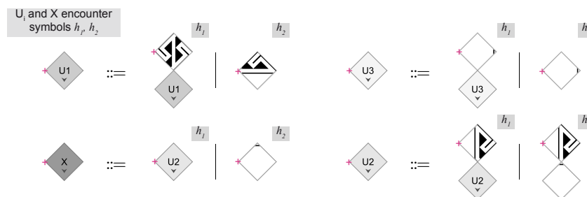
Figure 10: Transducer rules to produce the second type of corner
