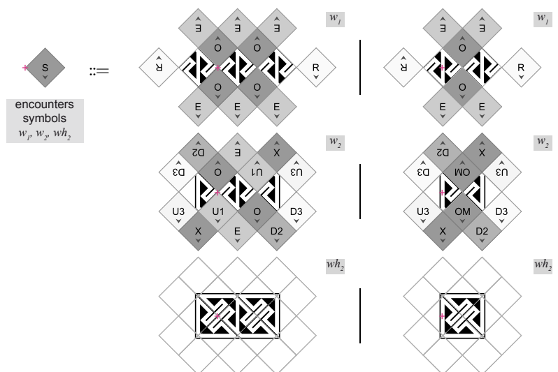
Figure 6: Transducer rules to start a computation from the initial state
