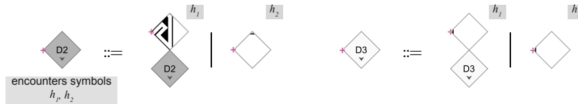
Figure 9: Transducer rules to grow the vertical borders
