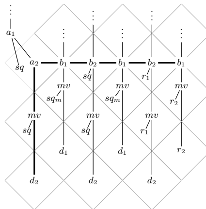
Figure 4: A sketch of a tree over collage operations that generates the lower right section of the key pattern in Figure 2
